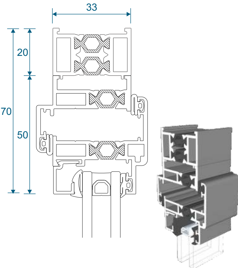
SW0001-0002 With 20mm Extension
