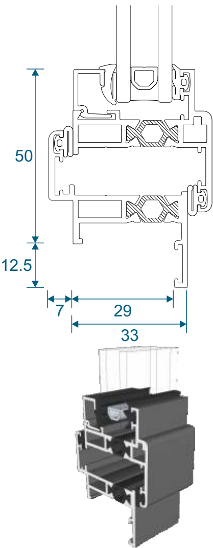
SW0001-0003 - Odd Leg
