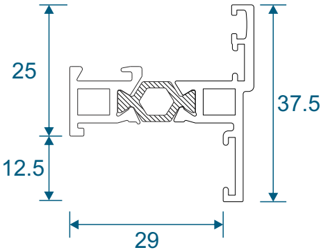
SW0001-0003 - Opener Odd Leg
