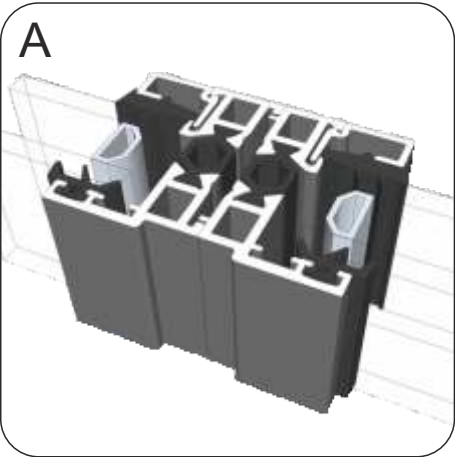
Using Hidden Coupler
