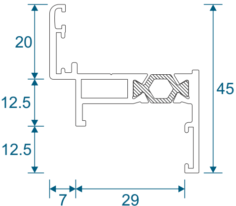
SW0001-0003 - Opener Odd Leg
