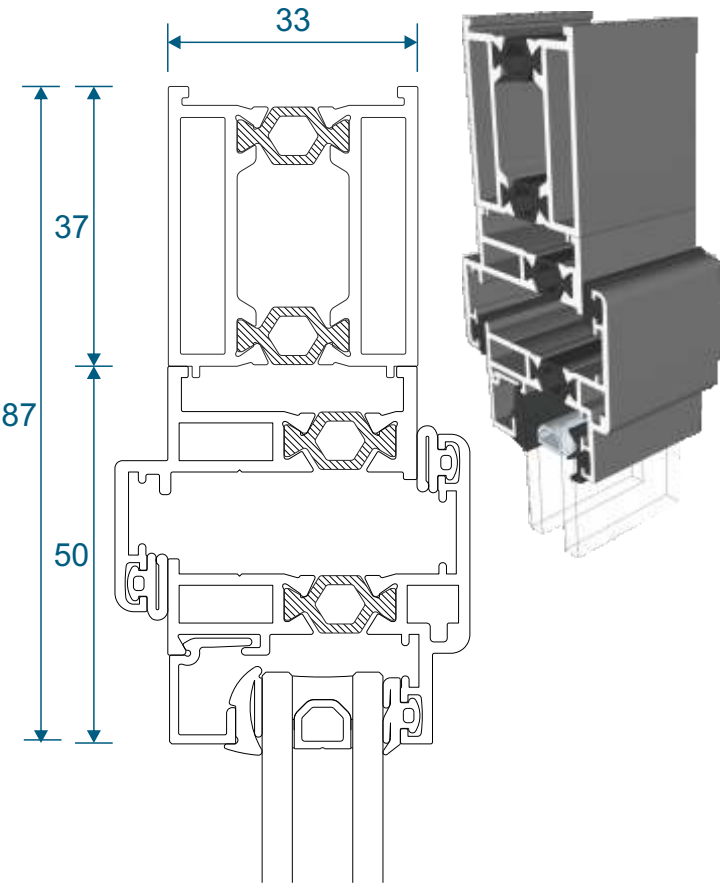
SW0001-0002 With 20mm Extension
