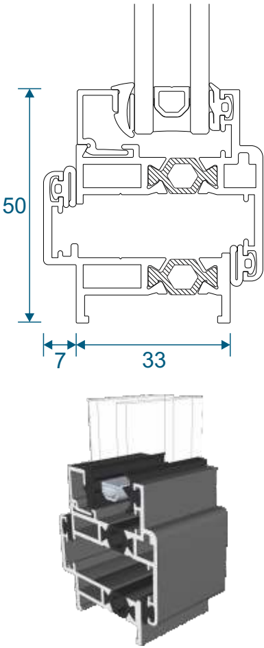
SW0001-0002 - No Cill
