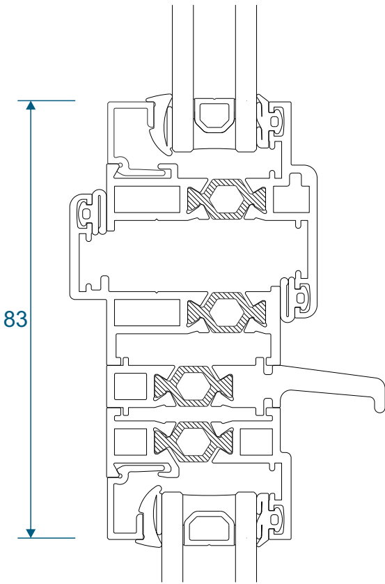
Opener Over A Fixed
