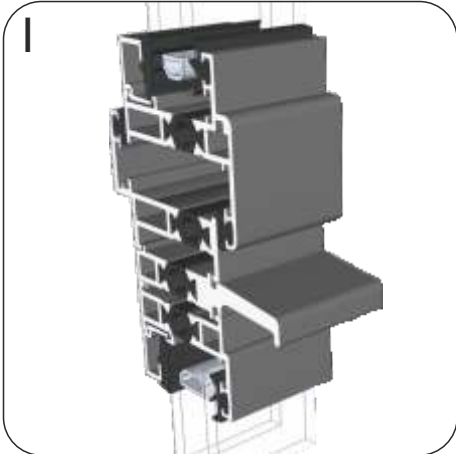
Using Drip Bar Coupler
