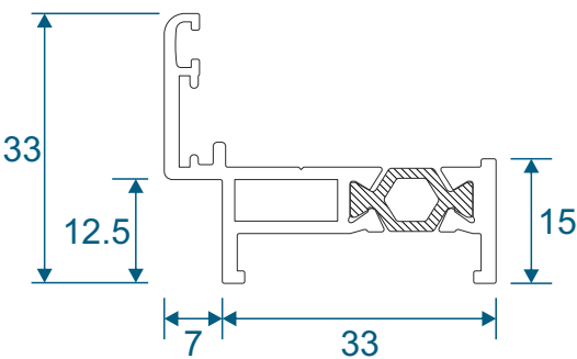
SW0006-0008 - Fixed Odd Leg
