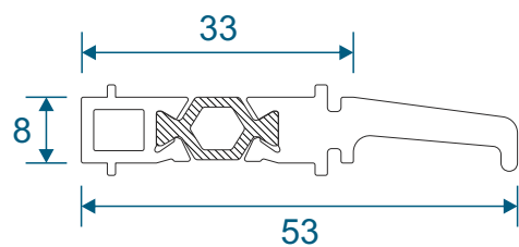
SW0017-0016 - Horizontal Drip Bar Coupler
