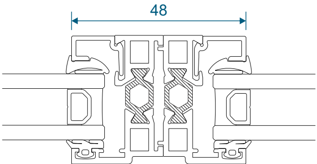
Fixed Next To Fixed
