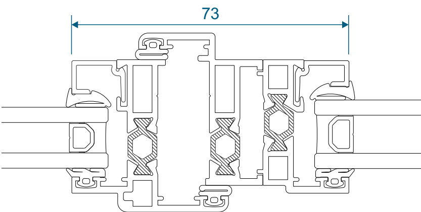
Opener Next To Fixed
