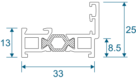
SW0001-0002 - Opener Equal Leg
